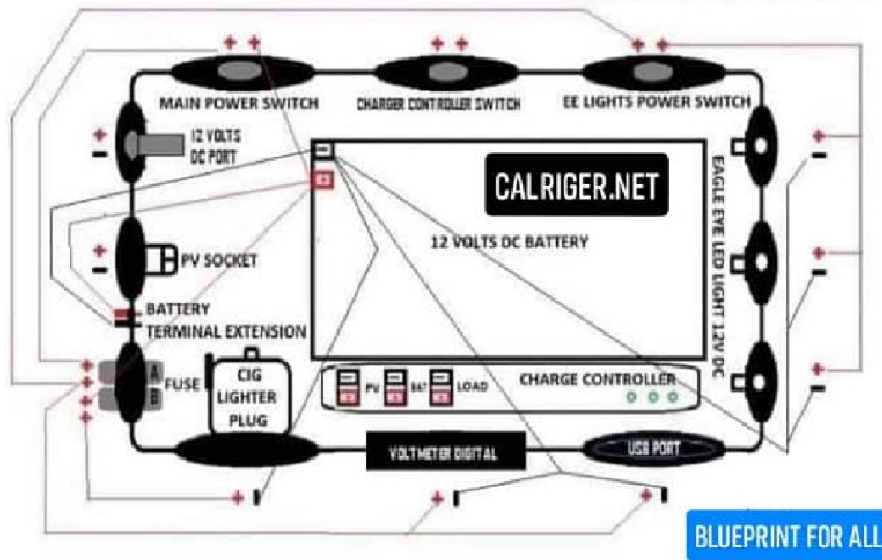
CALRIGER SOLARREV S1-GA10 DIAGRAM
